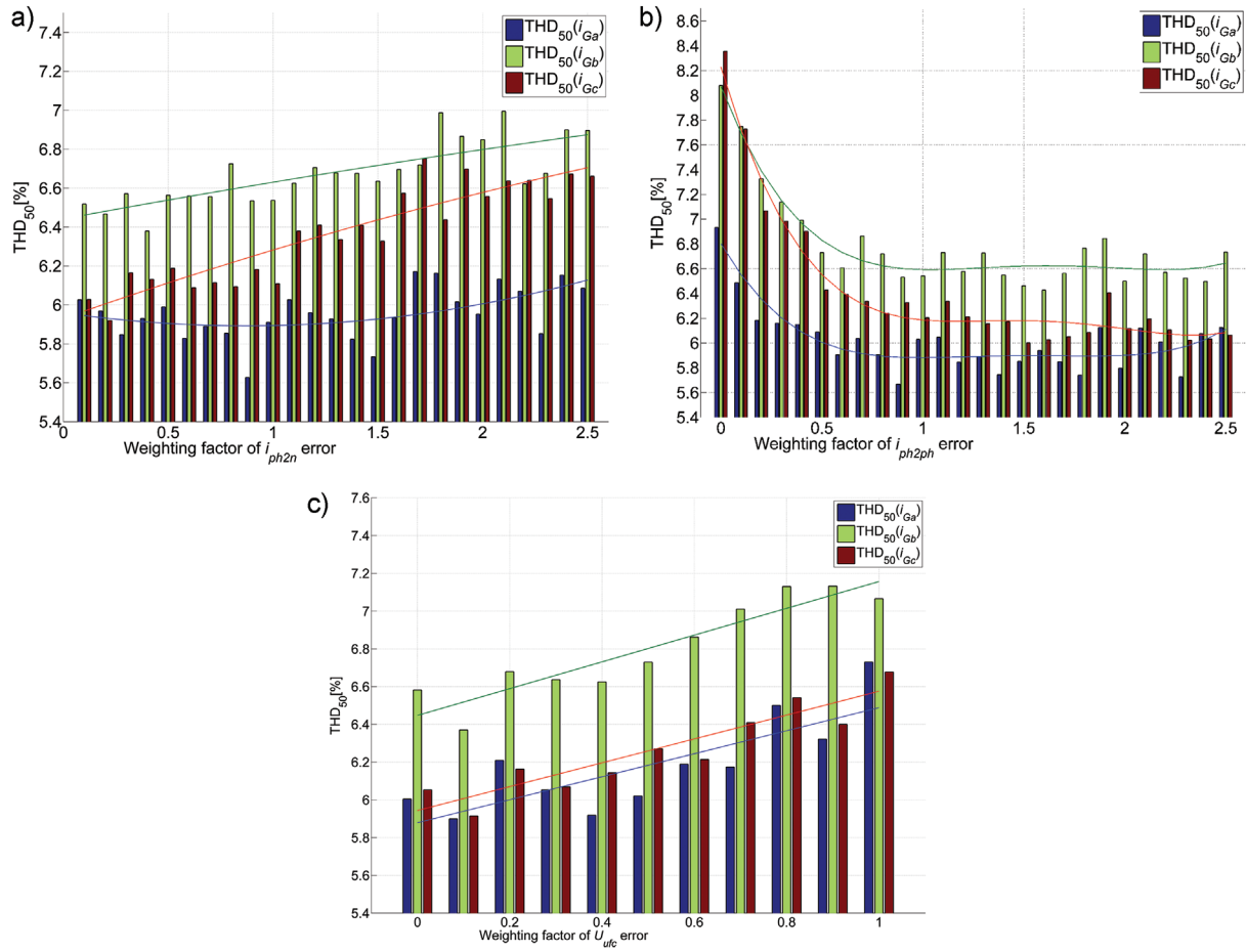
Fig. 6. The effect of change in the weight coefficients on the THD coefficient of the grid currents with regard to (a) w_{f1} (phase currents), (b) w_{f2} (line currents) and (c) w_{f_{U_{dre}}} (FC voltage errors)
