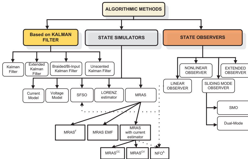
Fig. 1. Classification of induction motor state variables estimation methods (Tarchała et al., 2011)
