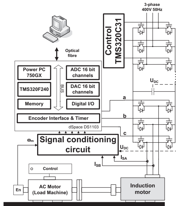
Fig. 10. Schematic diagram of the laboratory test bench (Dybkowski and Orlowska-Kowalska, 2012)
