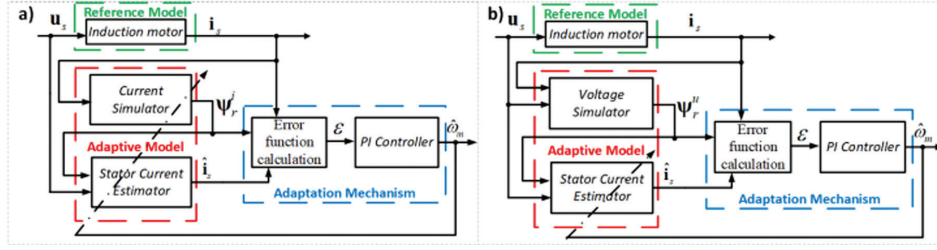
Fig. 1. The block diagrams of selected speed estimators: a) \text{MRAS}^{\text{CC}} , b) \text{MRAS}^{\text{CV}}
