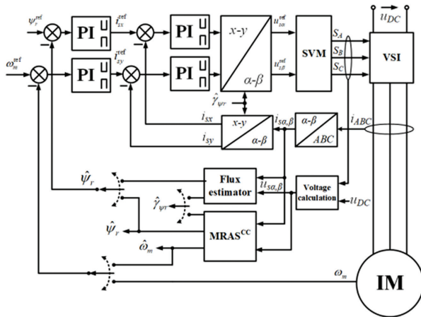
Fig. 5. Block diagram of the DFOC structure for the IM with MRAS estimators
