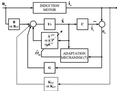
Fig. 2. The generalized block diagram of AFO, \text{MRAS}^{\text{CC}} and \text{MRAS}^{\text{CV}} speed estimators (matrix \mathbf{K}_{\text{CC}} or \mathbf{K}_{\text{CV}} and \mathbf{B}_{\text{CV}} appear only in \text{MRAS}^{\text{CC}} or \text{MRAS}^{\text{CV}} , respectively)
