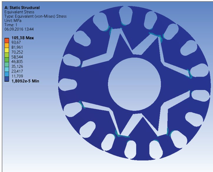
Fig. 3. Mechanical analyses of rotor sheet under stress: n_{\text{rotor}} = 1.2n , T_{\text{load}} = 20 T_n
