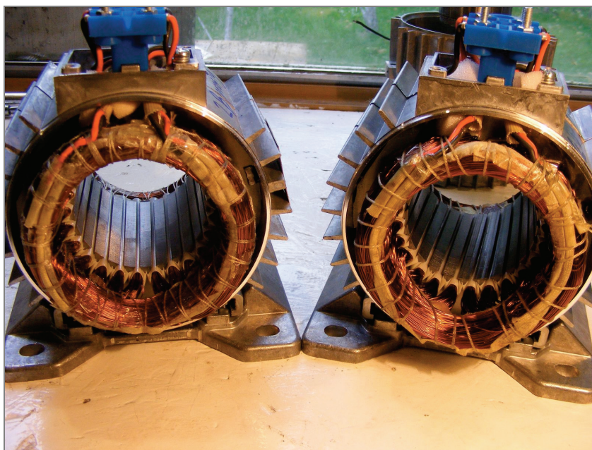
Fig. 5. Stators of the built motors: unskewed (left) and skewed (right)
