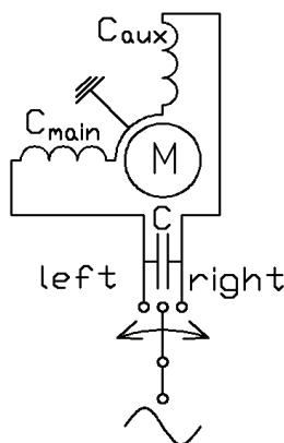
Fig. 6. Electrical scheme of the two-directional single-phase AC motor
