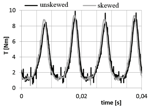
Fig. 10. Torques in time domain for the skewed and unskewed motor stator (rated load)
