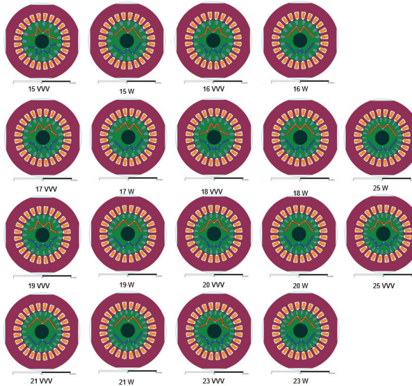
Fig. 1. Field parts of the field-circuit single-phase line start permanent magnet synchronous motor models
