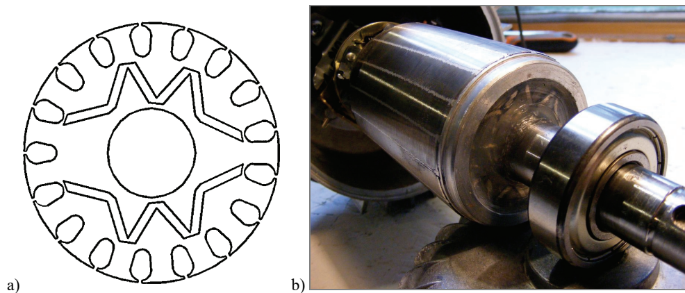
Fig. 4. Rotor with interior permanent magnets and aluminium die-cast cage: (a) rotor sheet cross section, (b) rotor before assembly into stator
