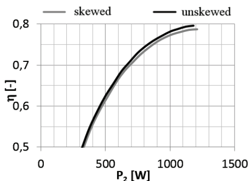
Fig. 7. Efficiency curves for the skewed and unskewed motor stator
