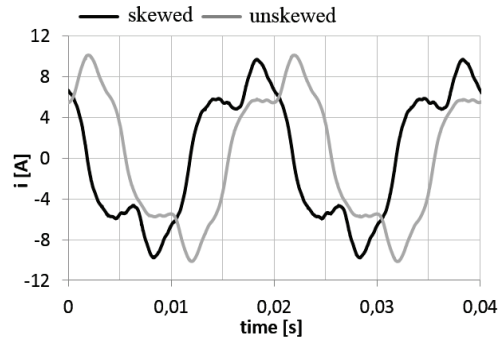
Fig. 9. Currents in time domain for the skewed and unskewed motor stator (rated load)
