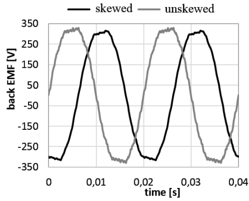
Fig. 8. Back EMFs in time domain for the skewed and unskewed motor stator (idle running)
