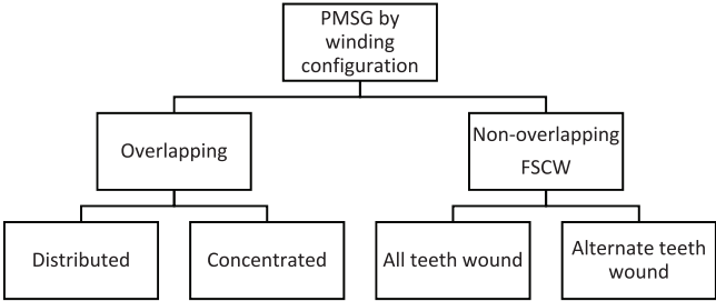
Fig. 1. Radial PMSG stator topologies [6]
